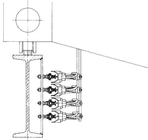
Lateral arrangement of the conductor rails. Only in dry and dust free halls possible. Lateral arrangement preferably with CH-profiles
