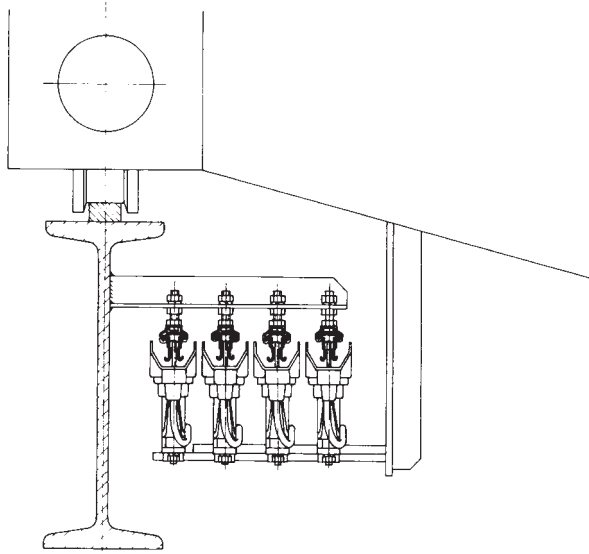
Suspended mounting of 4-pole system.
